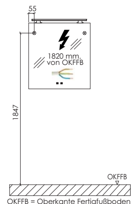
FSB 40xx B/C1
